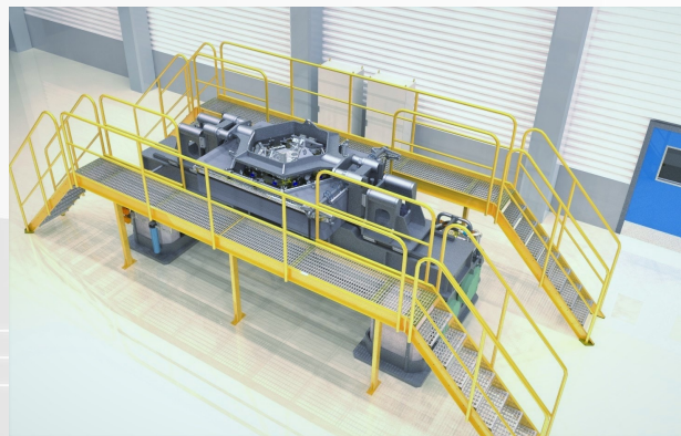
ESO ELT – Washing and Stripping Plant
