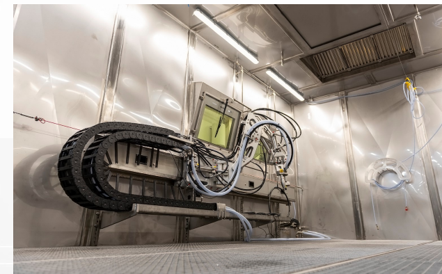
Nuclear Decontamination Remote Manipulator
